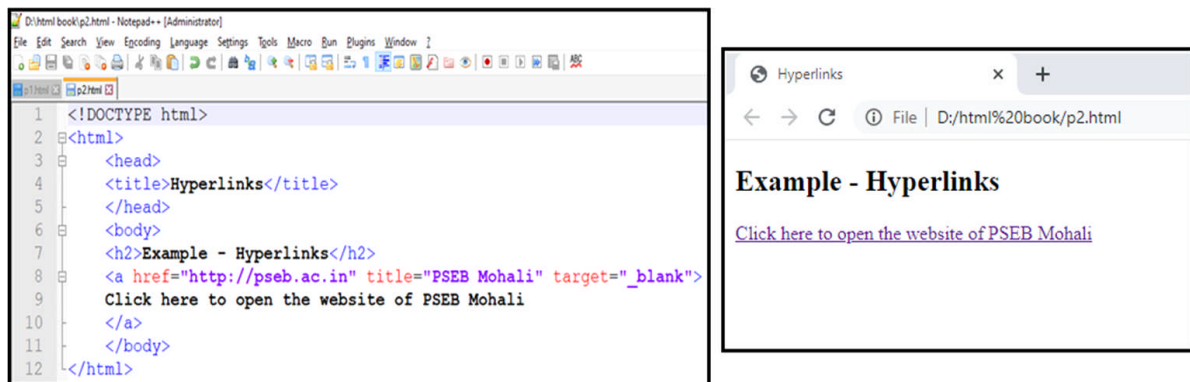
Figure 1.5 - HTML Code for creating Hyperlinks and Its output window
